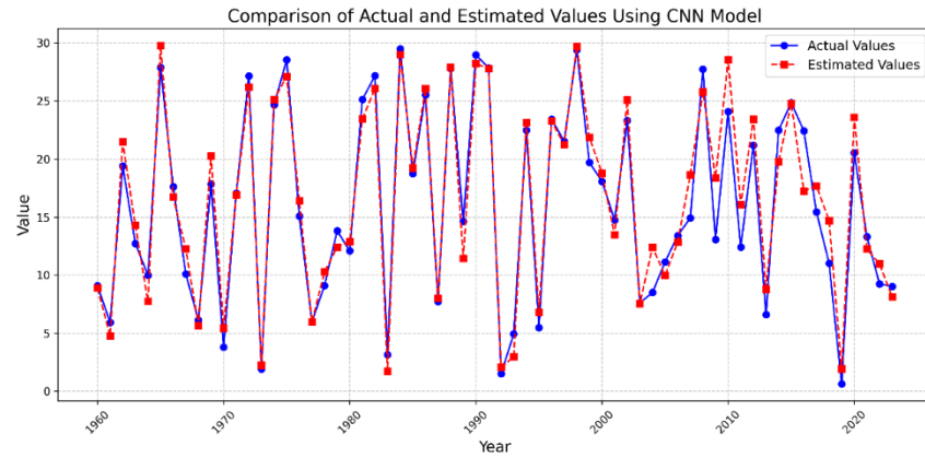
Fig. 4. Model Performance Comparison (Actual vs. Estimated)
