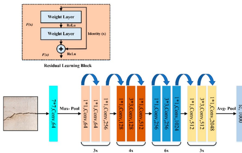
Fig 1: Architecture of ResNet50 Pre-trained CNN [8]
