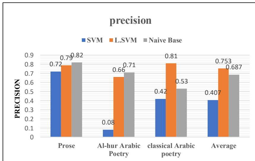
Fig. 7. Precision for SVM, LSVM and Naive Base Algorithms
