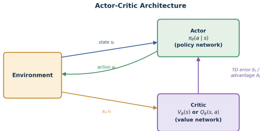
Fig. 4. Actor-critic architecture.
