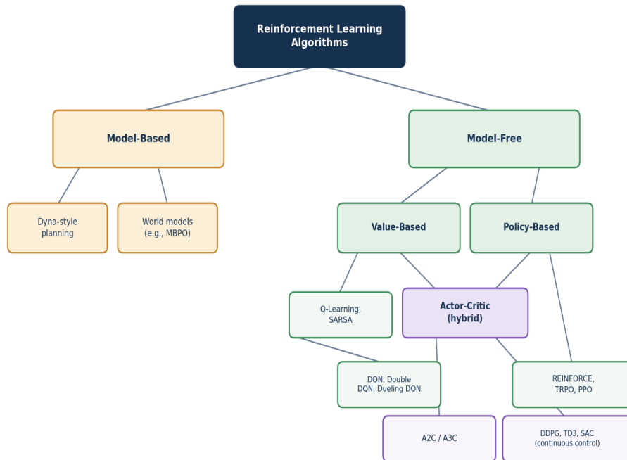
Fig. 1. Taxonomy of reinforcement learning algorithms by the source of the training signal.
