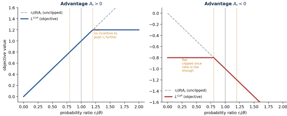
Fig. 3. PPO’s clipped surrogate objective, L^{\text{CLIP}} , as a function of the policy probability ratio r_t(\theta) , shown positive advantages on the left and negative advantages on the right. The objective becomes flat when r_t(\theta) moves \epsilon away from 1 in the favorable direction, removing the incentive for arbitrarily large policy updates while preserving the gradient for corrective updates in the unfavorable direction.
