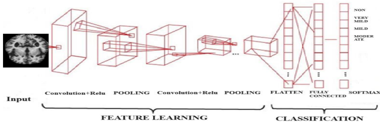
Fig. 2. CNN Architecture.
