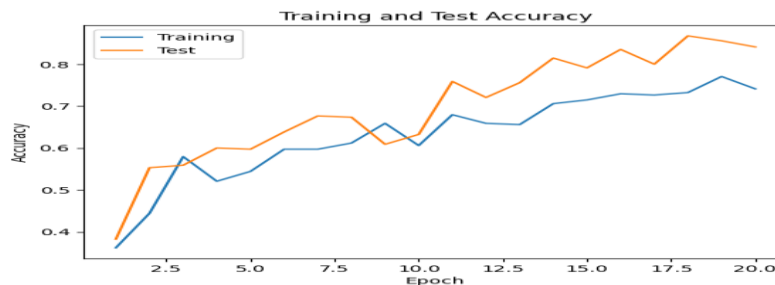
Fig. 6. Model Training
