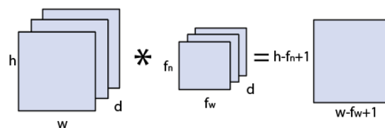
Fig. 3. Working of Operation of Convolution
