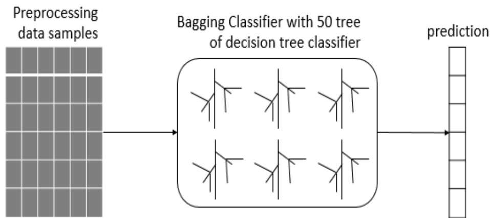
Fig 7. Proposed model.
