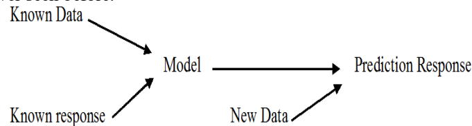
Fig 2. Supervised Learning.
