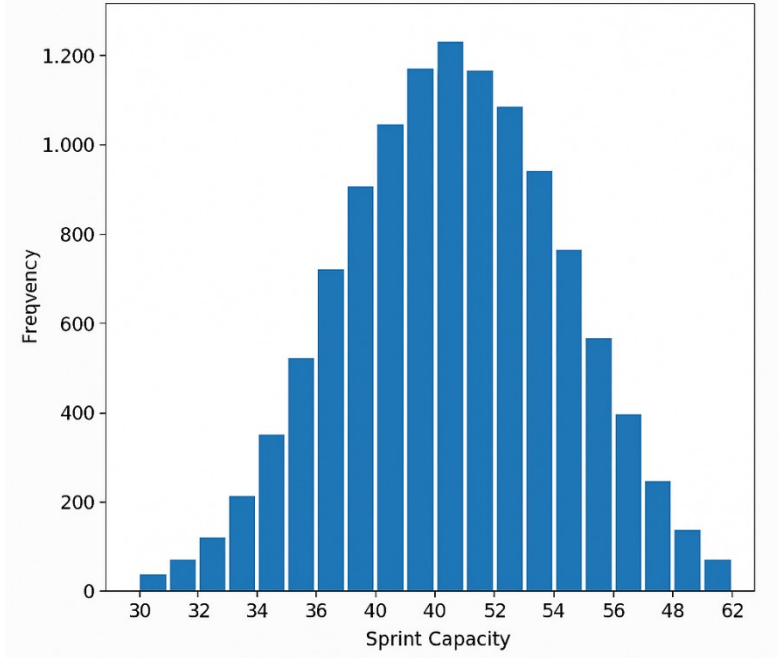
Fig. 2. Monte Carlo Sprint Forecasting Histogram
