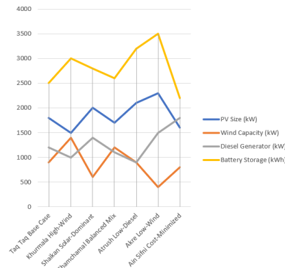
Fig. 4. Hybrid System Optimization (HOMER-Pro Output Summary)
