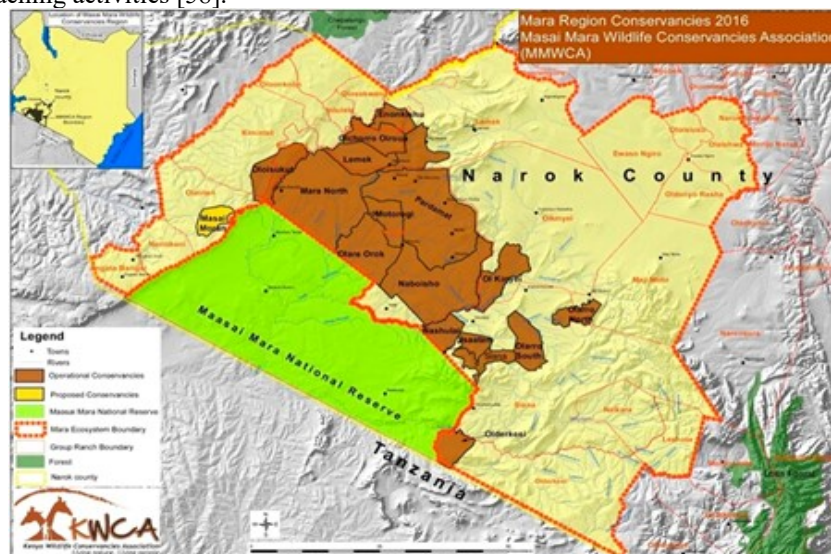
Fig. 4. A case study area map showing the Maasai Mara National Reserve which is part of the larger Maasai Mara-Serengeti Savanna Ecosystem (Adapted from KWCA).
