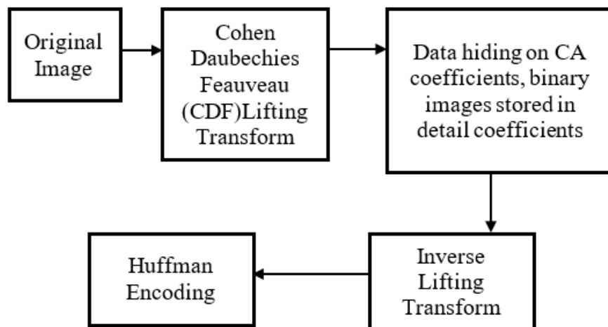
Fig. 7. Image steganography with Huffman algorithm [88].
