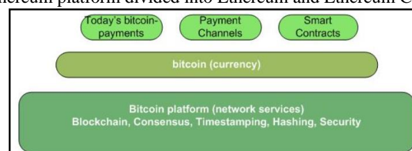
Fig .2. Bitcoin's layered architecture
