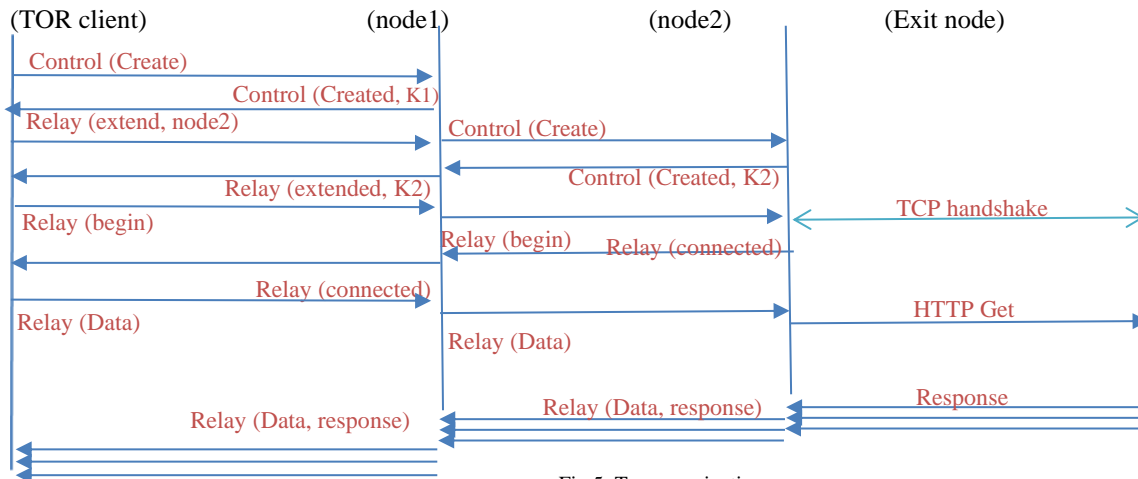
Fig 5: Tor connection
