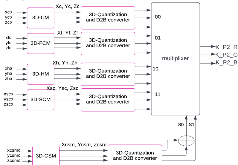
Fig. 1. Key generation Proposal, selection method (P2Sel)
