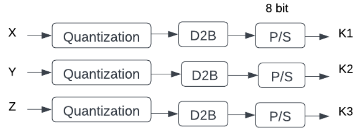
Fig. 2. 3D-Quantization and Decimal-to-binary converter block diagram
