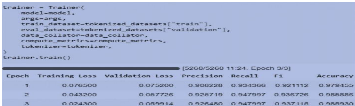
Fig .2. Evaluation results for BERT CONLL2003
