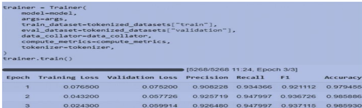
Fig .2. Evaluation results for BERT CONLEvaluation results for BERT CONLL2003
