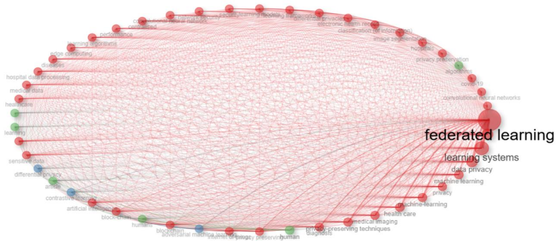
Fig 8 Co-Word Network
